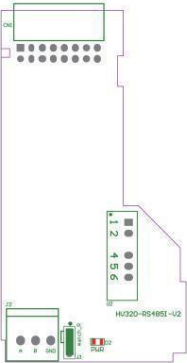
HV320-RS485I-V2 interface layout
